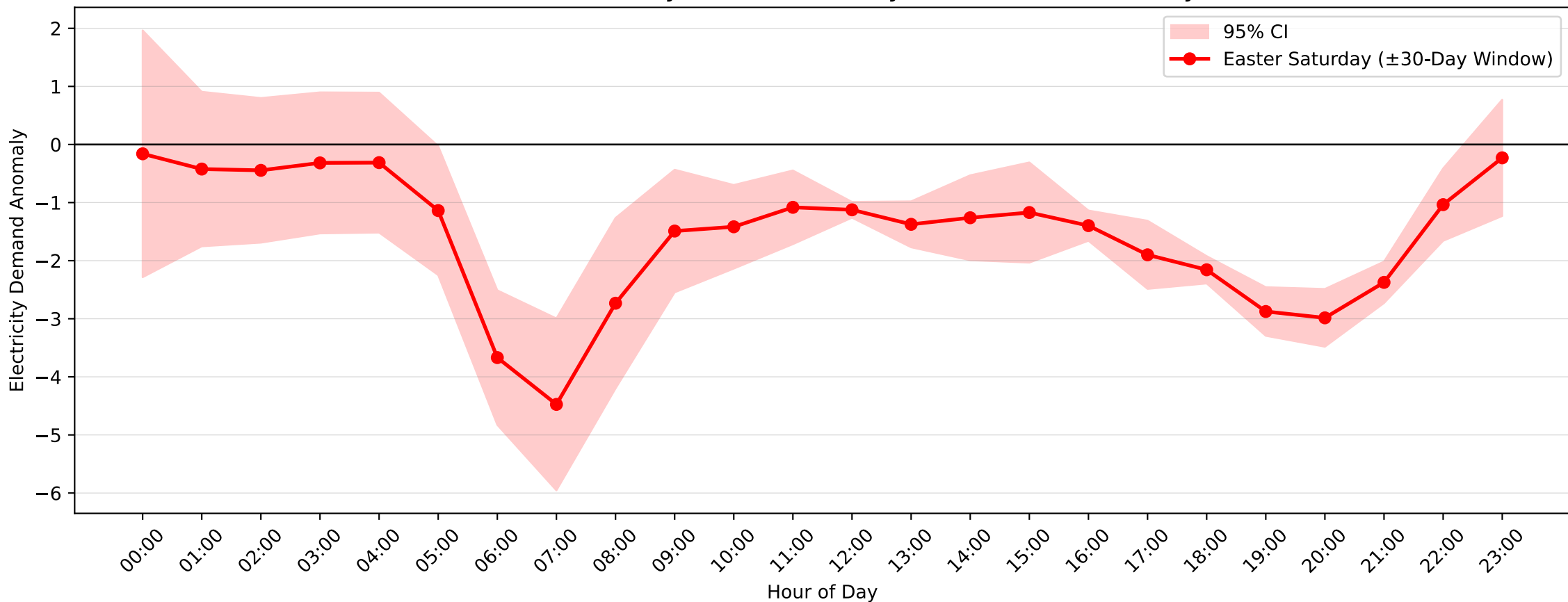
Mortdale Demand Anomaly: Easter Saturday (2011-2012, \pm 30 -Day Window)
