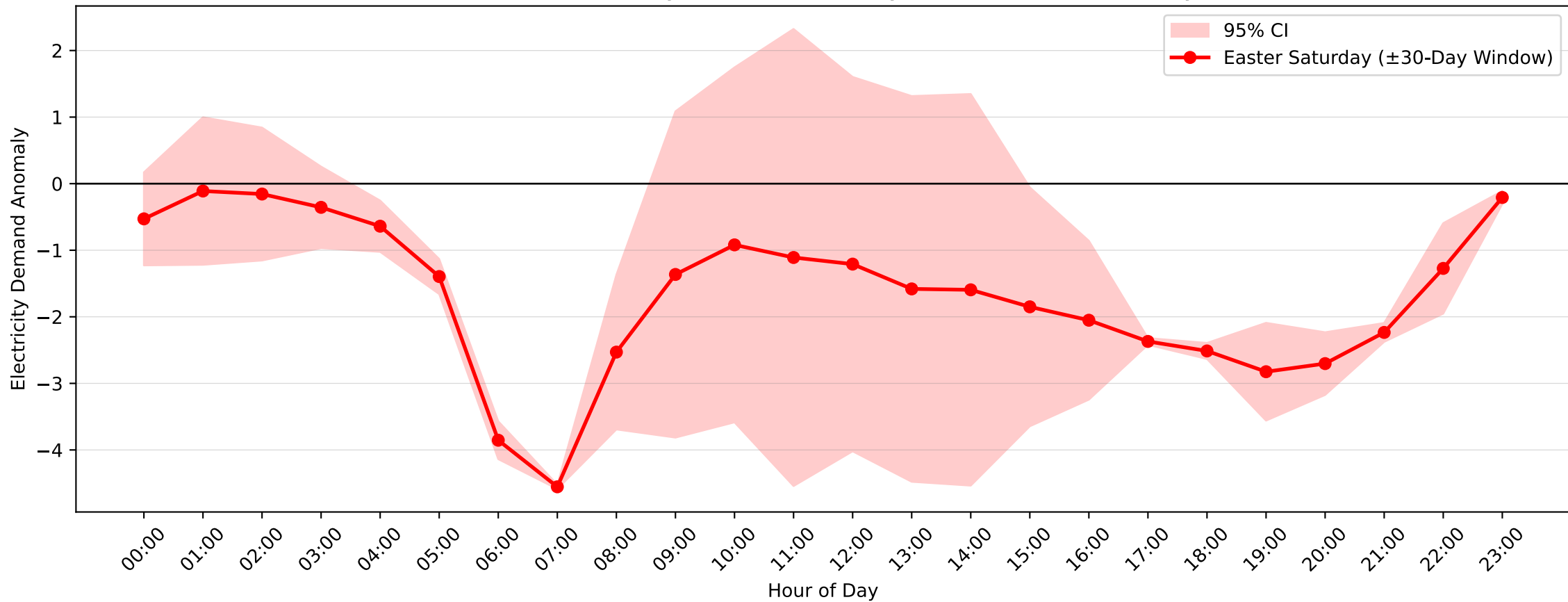
Mortdale Demand Anomaly: Easter Saturday (2014-2015, \pm 30 -Day Window)
